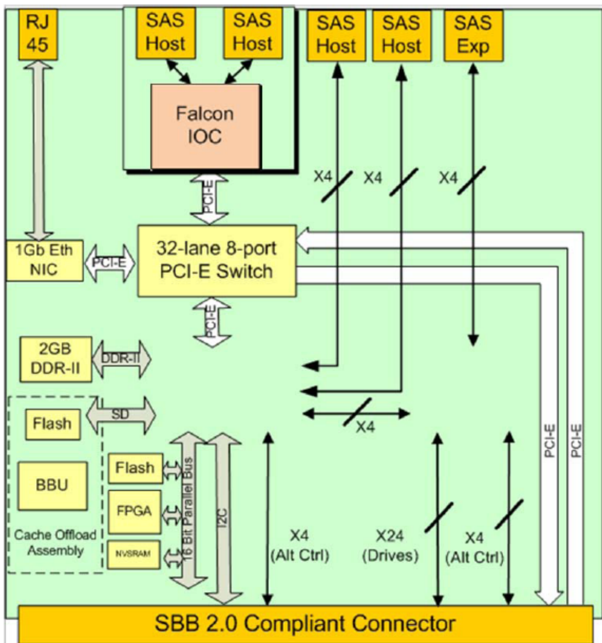
Figure 1. Controller Architecture
